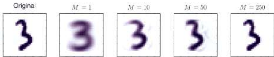
Figure 12.5 An original example from the off-line digits data set together with its PCA reconstructions obtained by retaining M principal components for various values of M . As M increases the reconstruction becomes more accurate and would become perfect when M = D = 28 \times 28 = 784 .
