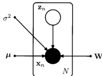
Figure 12.10 The probabilistic PCA model for a data set of N observations of \mathbf{x} can be expressed as a directed graph in which each observation \mathbf{x}_n is associated with a value z_n of the latent variable.
